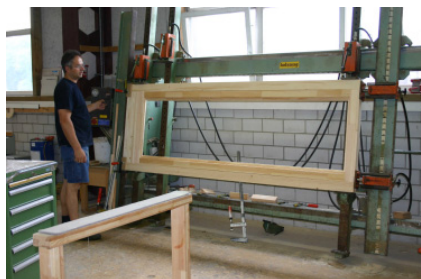
Stage 5 Glueing & jointing
